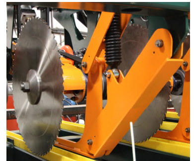
HOLD DOWNS WITH PARALLEL ARMS AND SHOCKS
