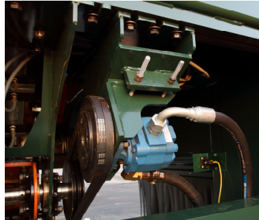
DUAL HYDRAULIC MOTORS OR DUAL 25 HP TEFC ELECTRIC MOTORS TO POWER LINE SHAFT
