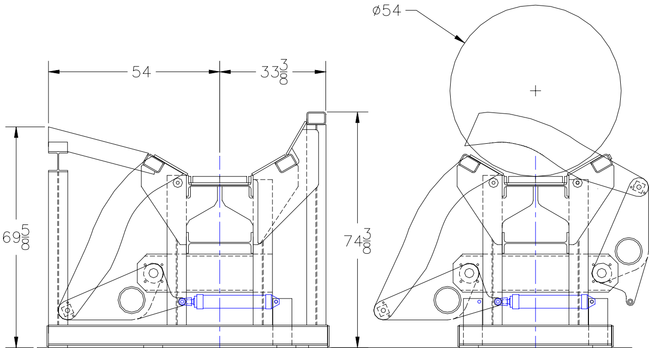
END VIEW WITH TRANSITION FROM DEBARKER AND REINFORCEMENT WITH BACKSTOP
